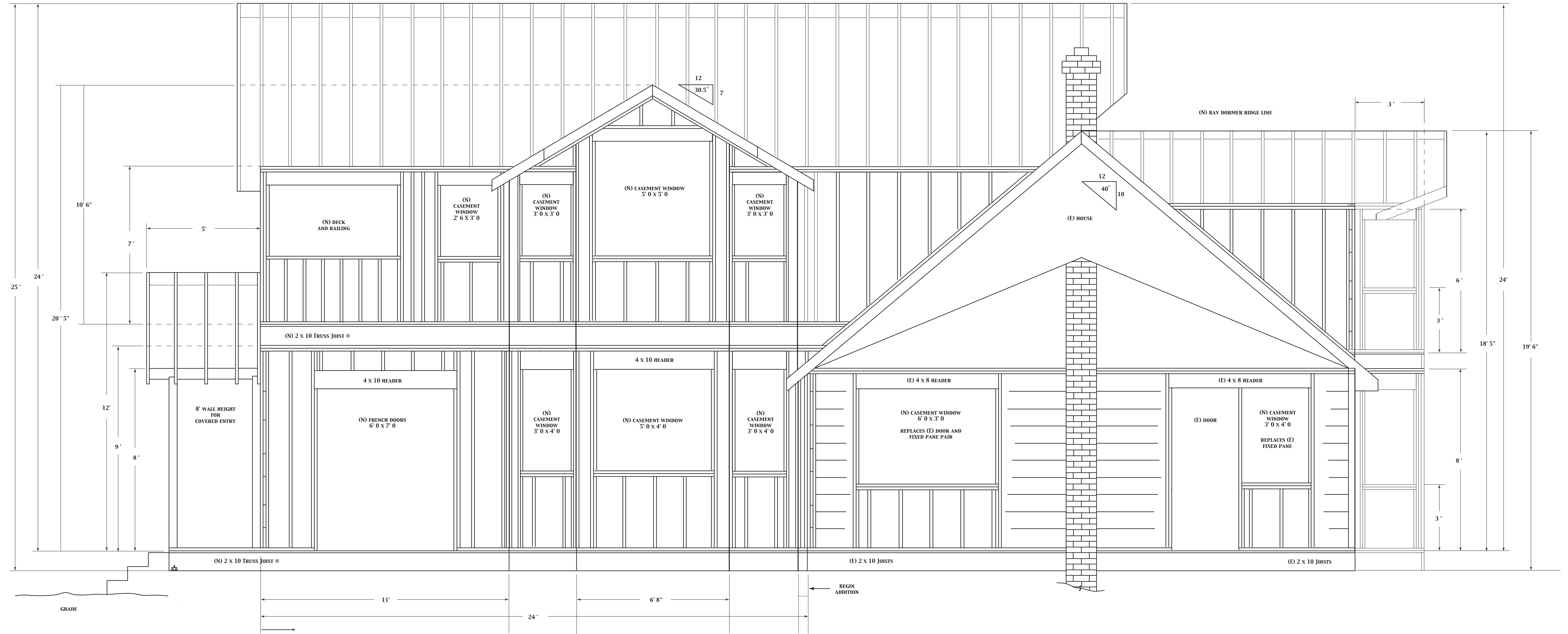
SOUTH ELEVATION AND WALL FRAMING PLAN
